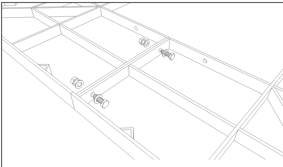
Pic. 3 Light Frame Bolts DIN933 M12 Rings DIN125 Nuts DIN985 M12
